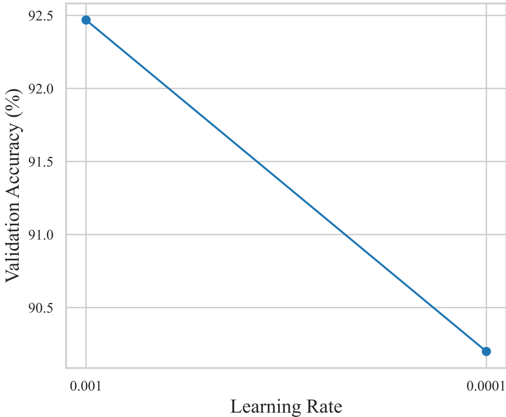
Plot 8: Learning Rate vs. Validation Accuracy
